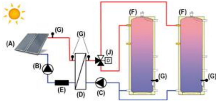
Management of two buffer tanks
