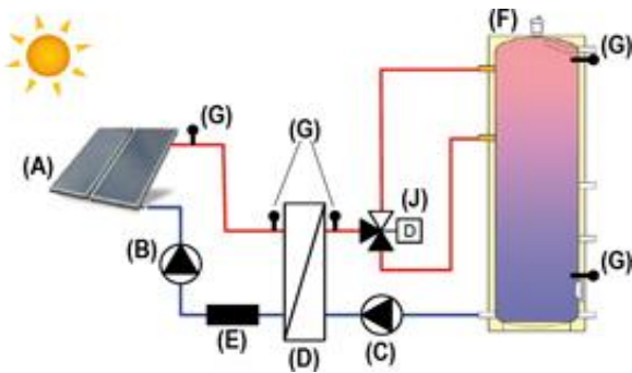
Management of one buffer tank loaded in stratification
