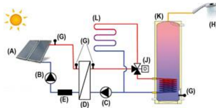
Heating and hot domestic water production
