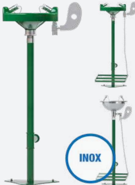
Ref. GW12 03 03 05 Recogedor en ABS ABS bowl Accionamiento con palanca o pedal Operated with push lever or pedal
