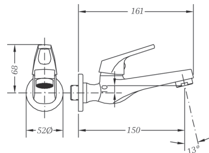
Grifo lavabo mural 1 agua cartucho 25 One-water wall wash-basin tap 25 cartridge
